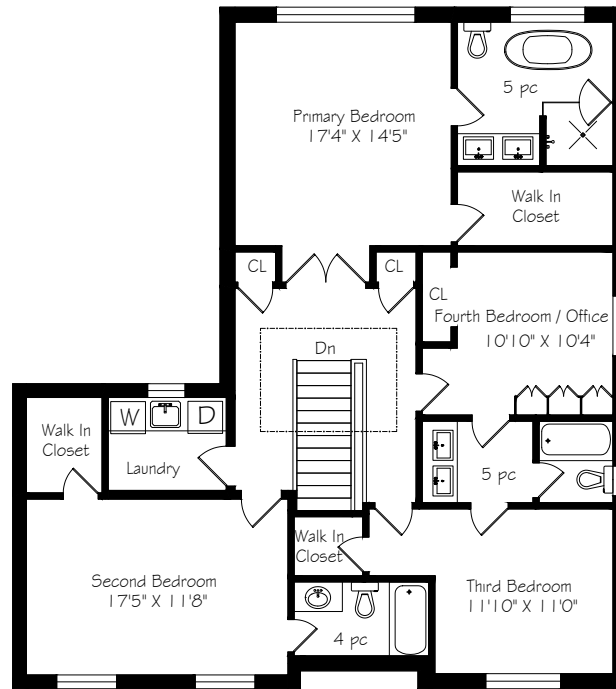
Second Floor 1506 Square Feet
