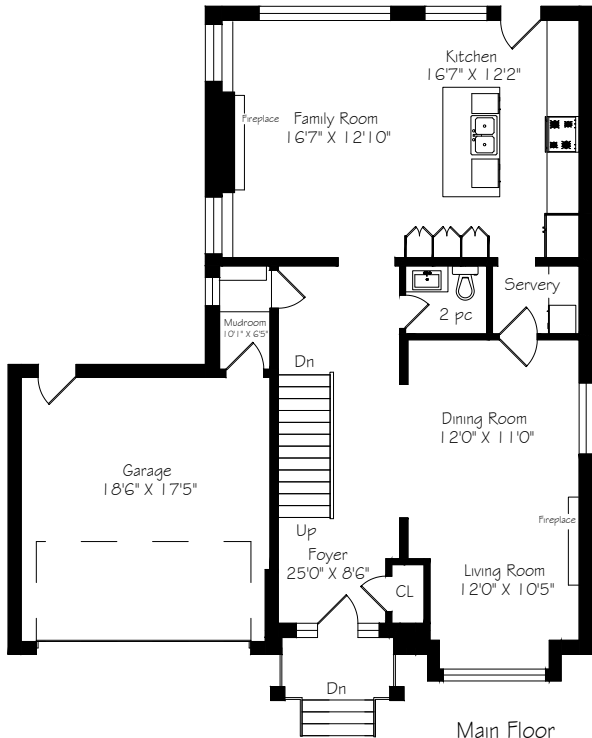
Main Floor 1154 Square Feet
